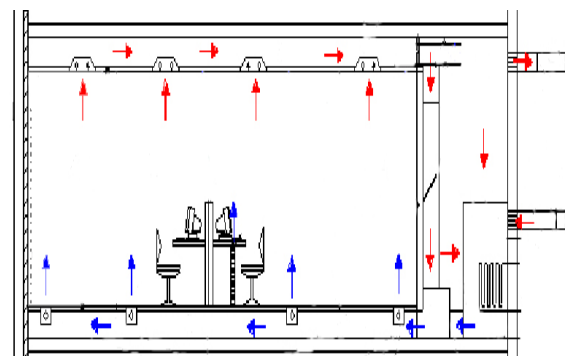
Fig. 1 – Schematic UFAD system – (Leite, 2003)
